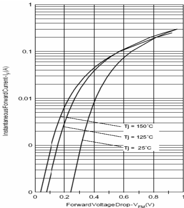
Fig. 1 - Max. Forward Voltage Drop Characteristics (Per Leg)
