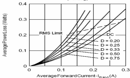
Fig. 4 - Forward Power Loss Characteristics
