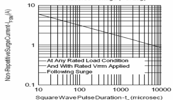
Fig. 5 - Max. Non-Repetitive Surge Current
