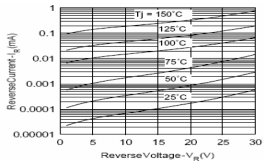
Fig. 2 - Typical Values Of Reverse Current Vs. Reverse Voltage (Per Leg)
